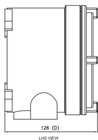
LHS VIEW
