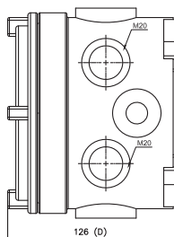
RHS VIEW
