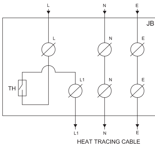
HEAT TRACING CABLE
